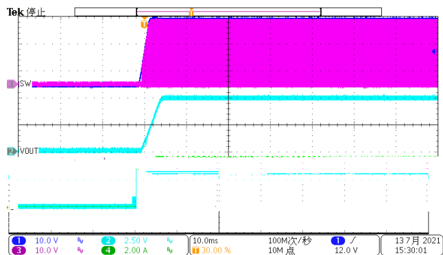
Figure 8. Power up(Iload=3A)
